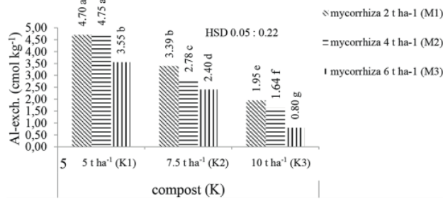
Fig. 9. Effect of the OPEFB compost and MVA on soil Al-exchangeable
